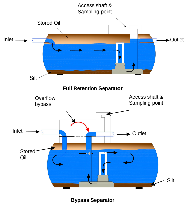
Figure 2.13 Typical Oil Separators
