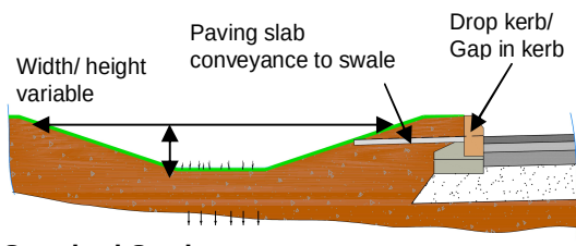
Standard Swale
