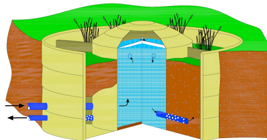
Figure 2.17 Retrofit Wetland Device
