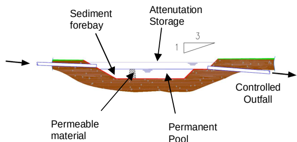
Indicative Section
