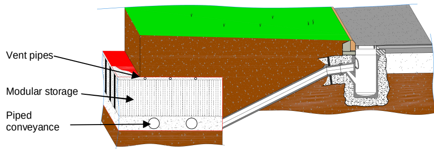
Figure 2.11 Modular Systems
