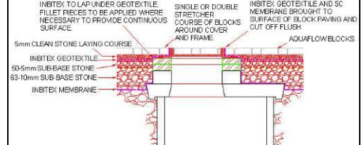
Figure 7. Pervious paving manhole detail
