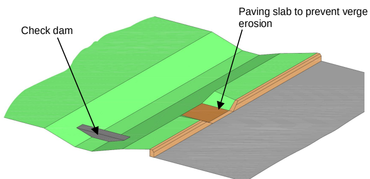
Swale Collecting Sheet Runoff
