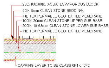
Figure 2. Pervious Paving Detail
