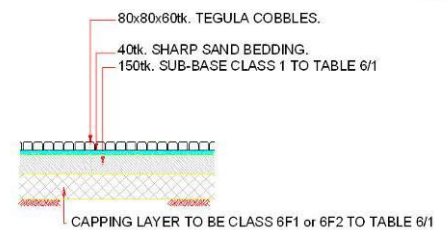
Figure 5. Services Strip (Tegula cobbles)
