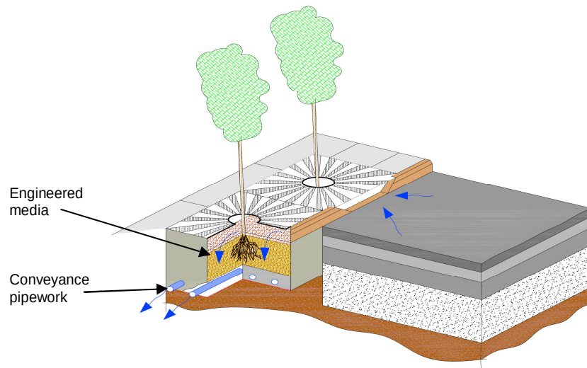
Figure 2.14 Prefabricated Bioretention
