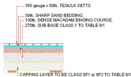
Figure 4. Services Strip (Tegula Setts)
