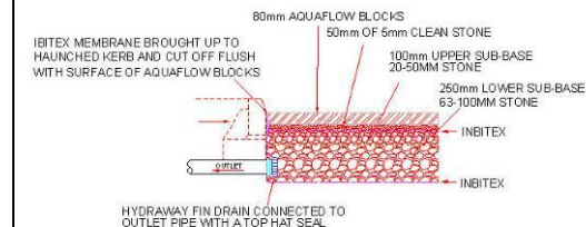
Figure 6. Pervious paving edge detail
