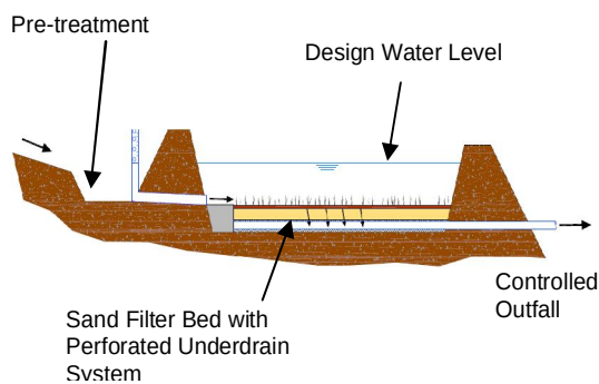
Indicative Section
