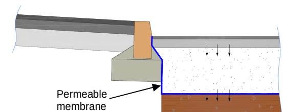
Indicative Section (With Infiltration)
