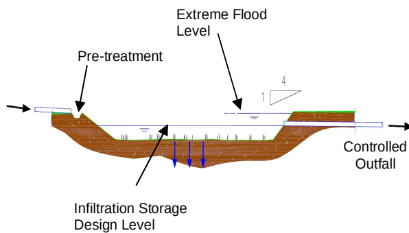
Indicative Section
