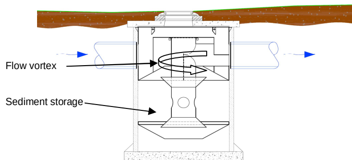
Figure 2.12 Hydrodynamic Separator
