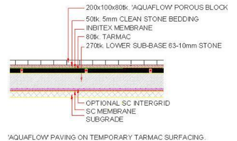
Figure 3. Pervious Paving over temporary construction (Aquaflow)
