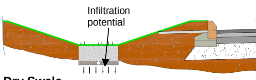
Dry Swale
