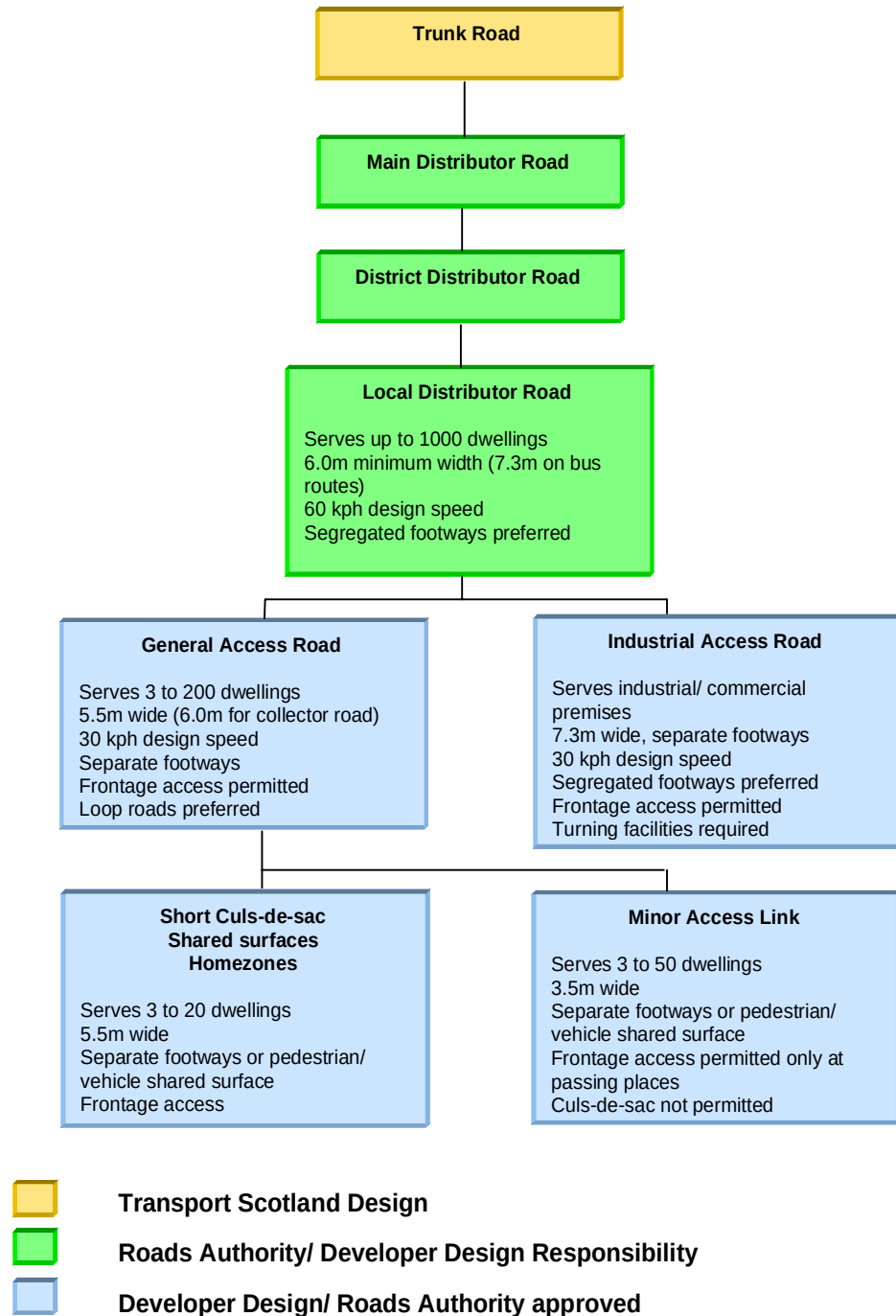
Figure 2.1 Illustration of Typical Traditional Road Hierarchy [2]
