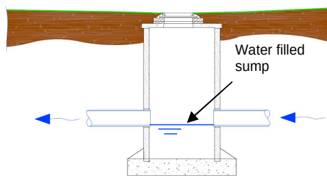
Indicative Section
